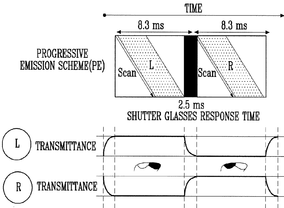
FIG. 3 (Related Art)
